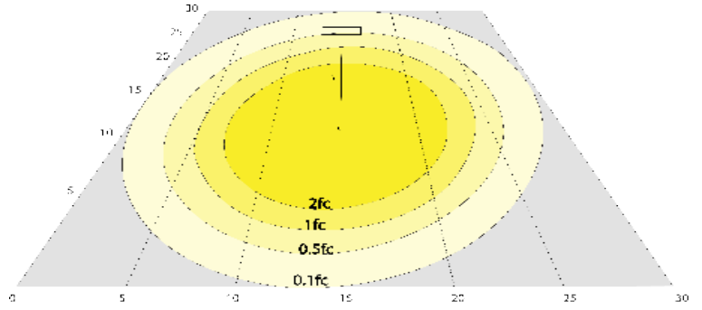
13W 3000K, Area 30'x 30' Mounting Height: 9'
